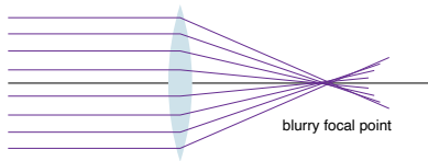
Spherical Aberrations
