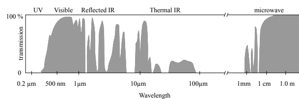
The transparency of the atmosphere
