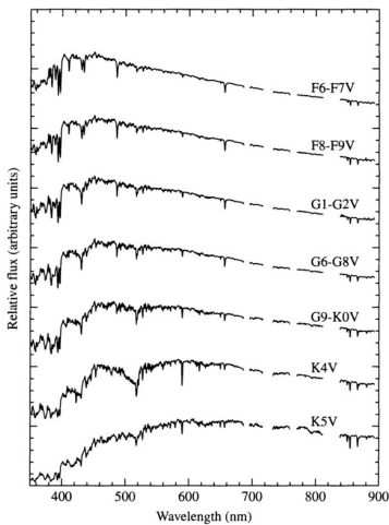
Spectra of main sequence stars
