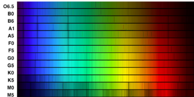
A more modern color spectrum showing the absorption lines from the various classes of stars.
